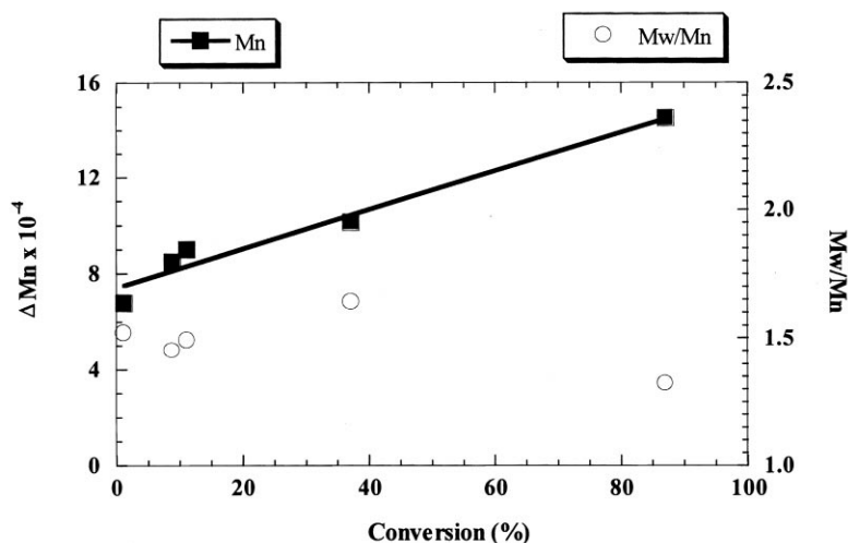
Fig. 2. Conversion versus molecular weight for MMA photopolymerization (room temperature fractions) by C-PTHF at \lambda = \sim 300 nm, \Delta M_n = M_{n_i} - M_{n_0} , C-PTHF = 0.2 g, MMA = 2 ml, \text{CH}_2\text{Cl}_2 = 2 ml, 25°C.
